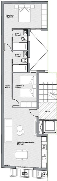
First Floor Apartment 1-A
